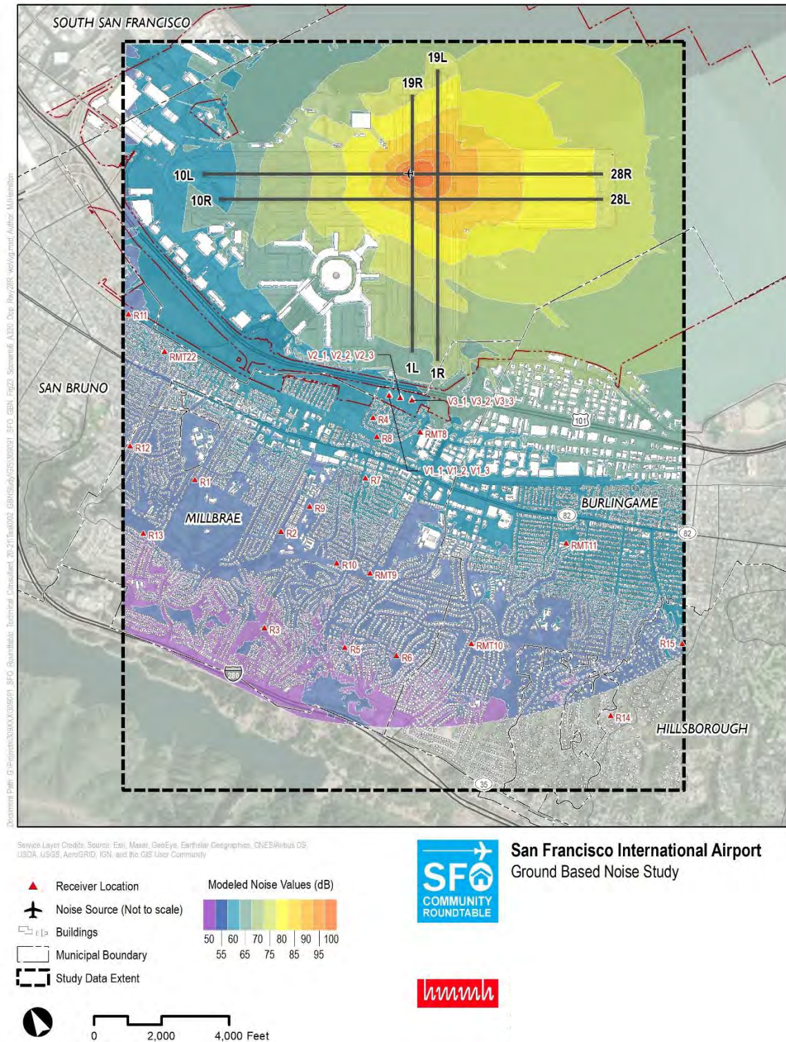
Figure 31: Scenario 6 – B738 Departing Runway 28R at Secondary Takeoff Point – Without Vegetation
