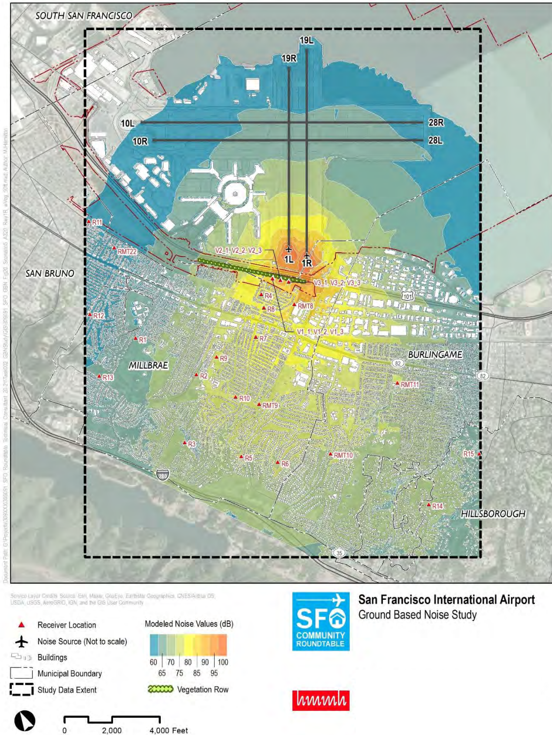
Figure 28: Scenario 5 – A320 Departing at the Same Time but Staggered on Runway 1L and 1R With Vegetation (50 Feet)
