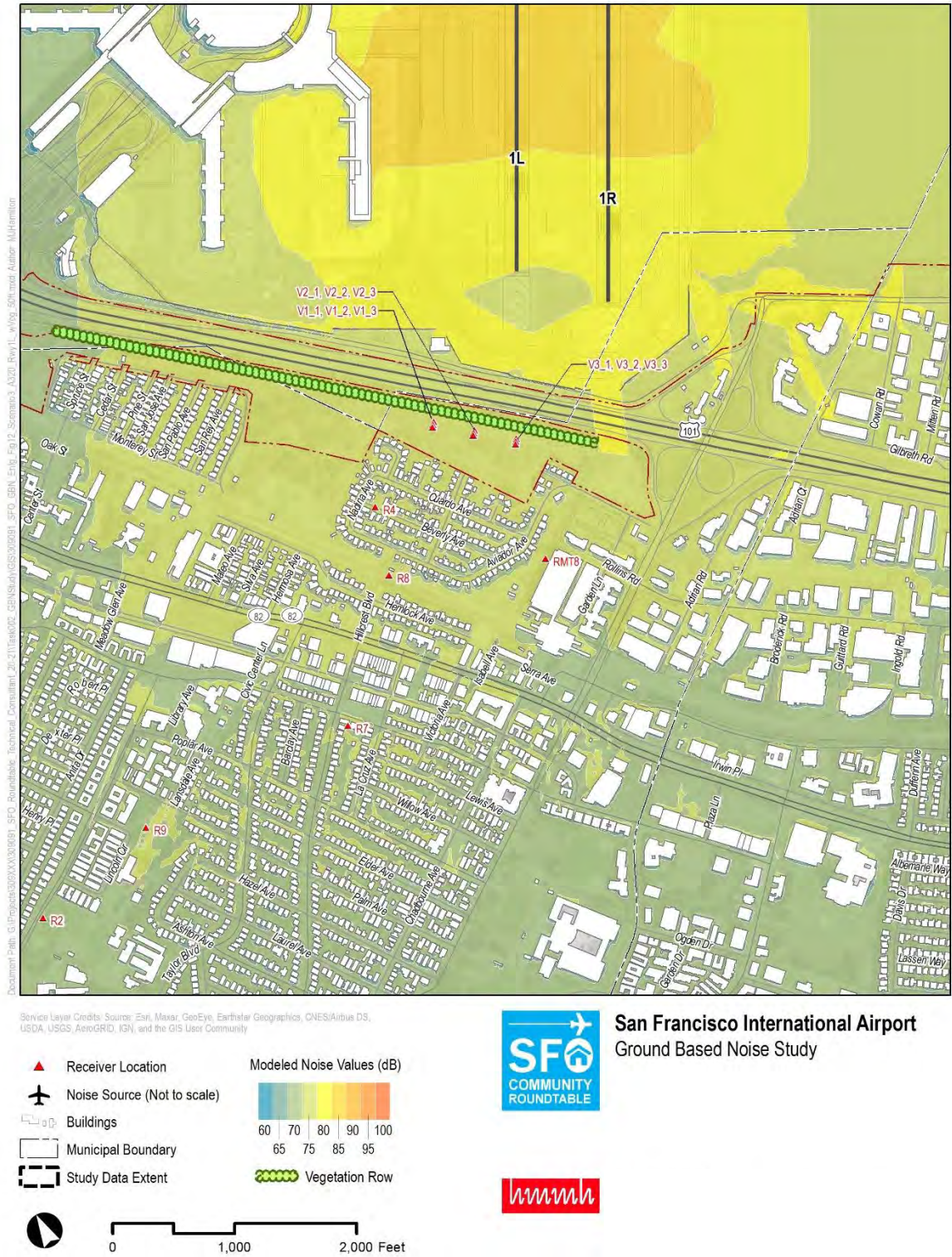
Figure H-12: Scenario 3 – A320 Departing Runway 1L at Secondary Takeoff Point – With Vegetation (50 Feet)
