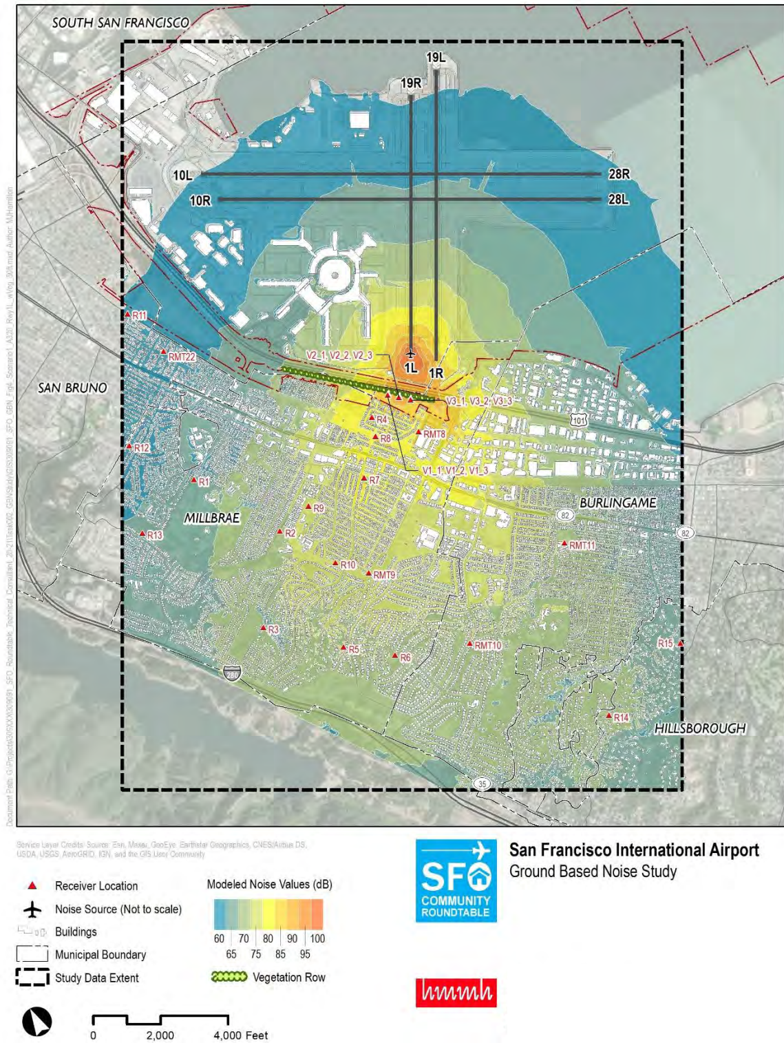
Figure 12: Scenario 1 – A320 Departing Runway 1L at Start of Takeoff Roll – With Vegetation (50 Feet)
