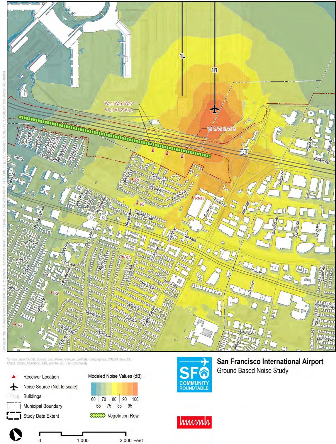
Figure H-8: Scenario 2 – A320 Departing Runway 1R at Start of Takeoff Roll – With Vegetation (50 Feet)
