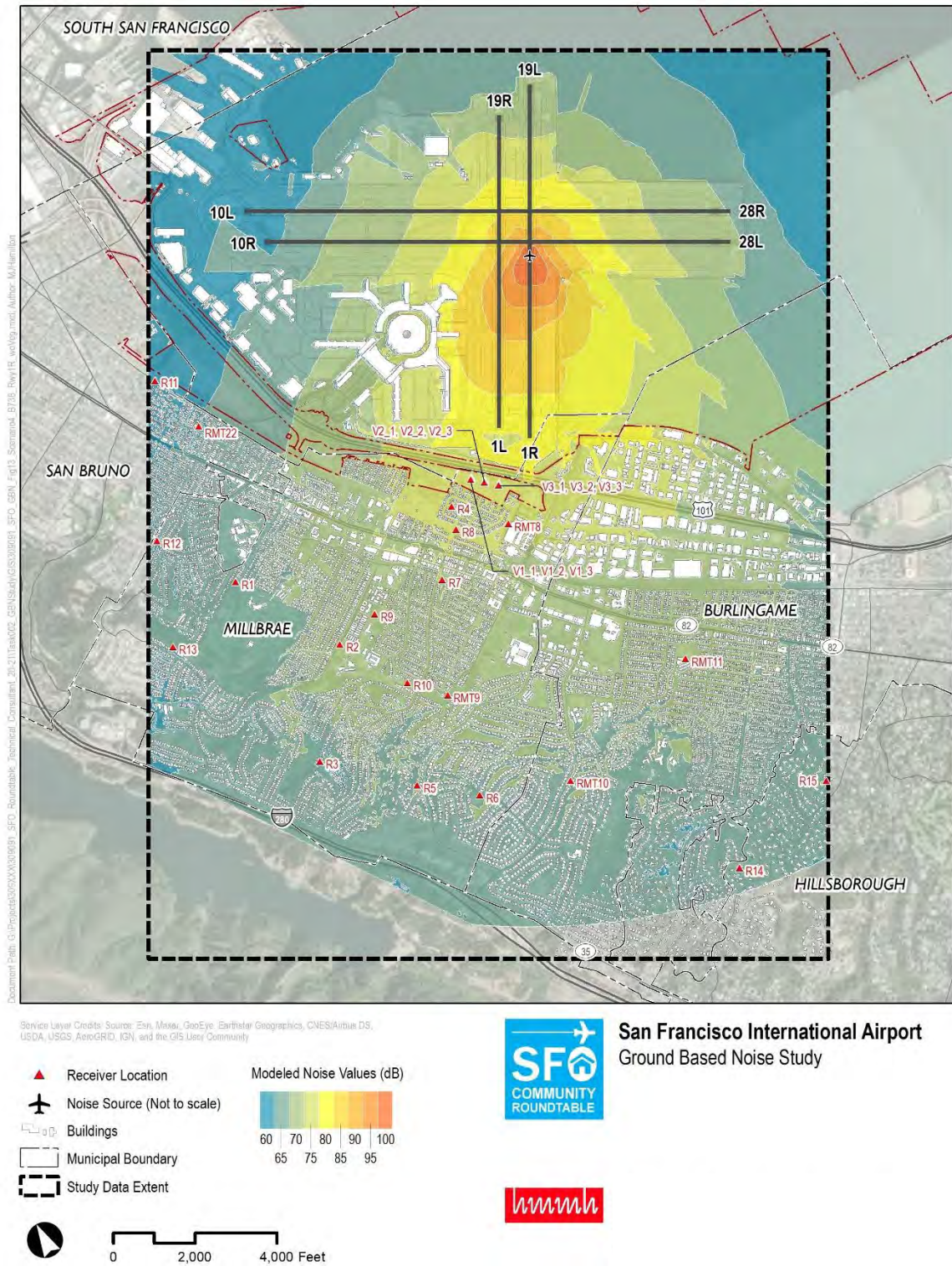
Figure 21: Scenario 4 – B738 Departing Runway 1R at Secondary Takeoff Point – Without Vegetation
