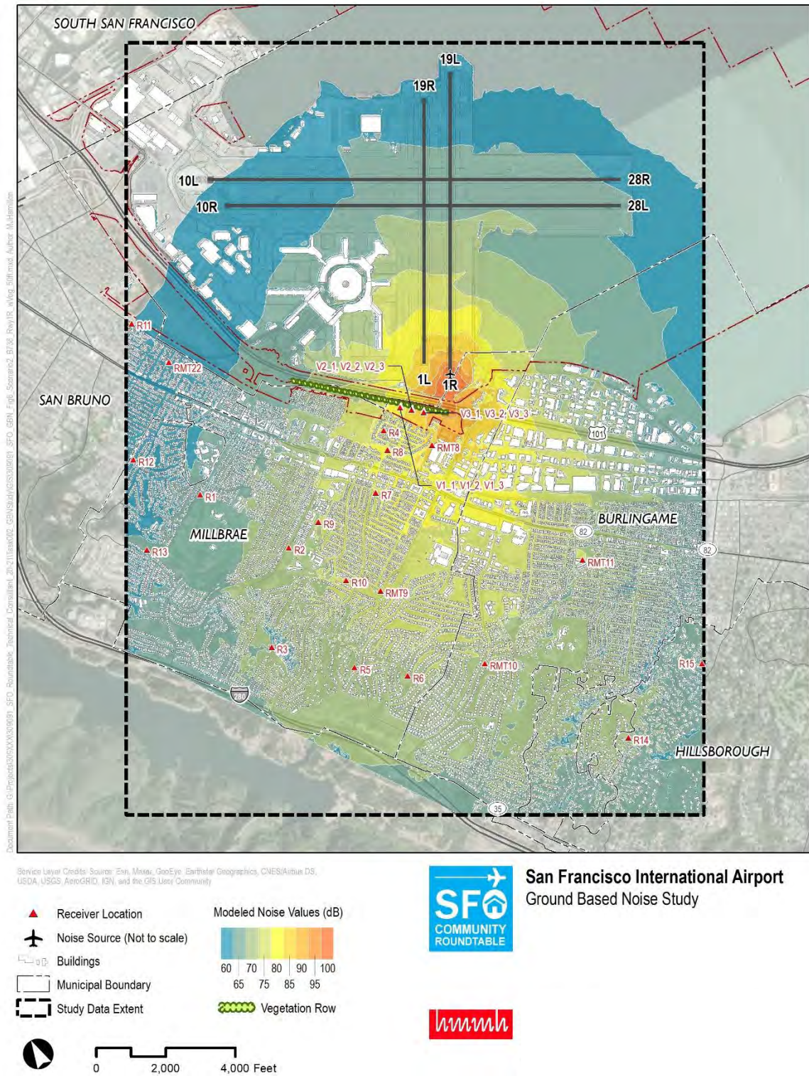
Figure 14: Scenario 2 – B738 Departing Runway 1R at Start of Takeoff Roll – With Vegetation (50 Feet)
