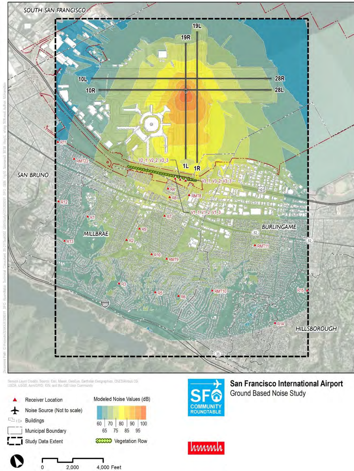
Figure 18: Scenario 3 – B738 Departing Runway 1L at Secondary Takeoff Point – With Vegetation (50 Feet)
