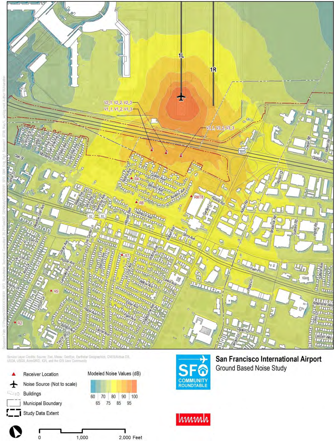
Figure H-1: Scenario 1 – B738 Departing Runway 1L at Start of Takeoff Roll – Without Vegetation
