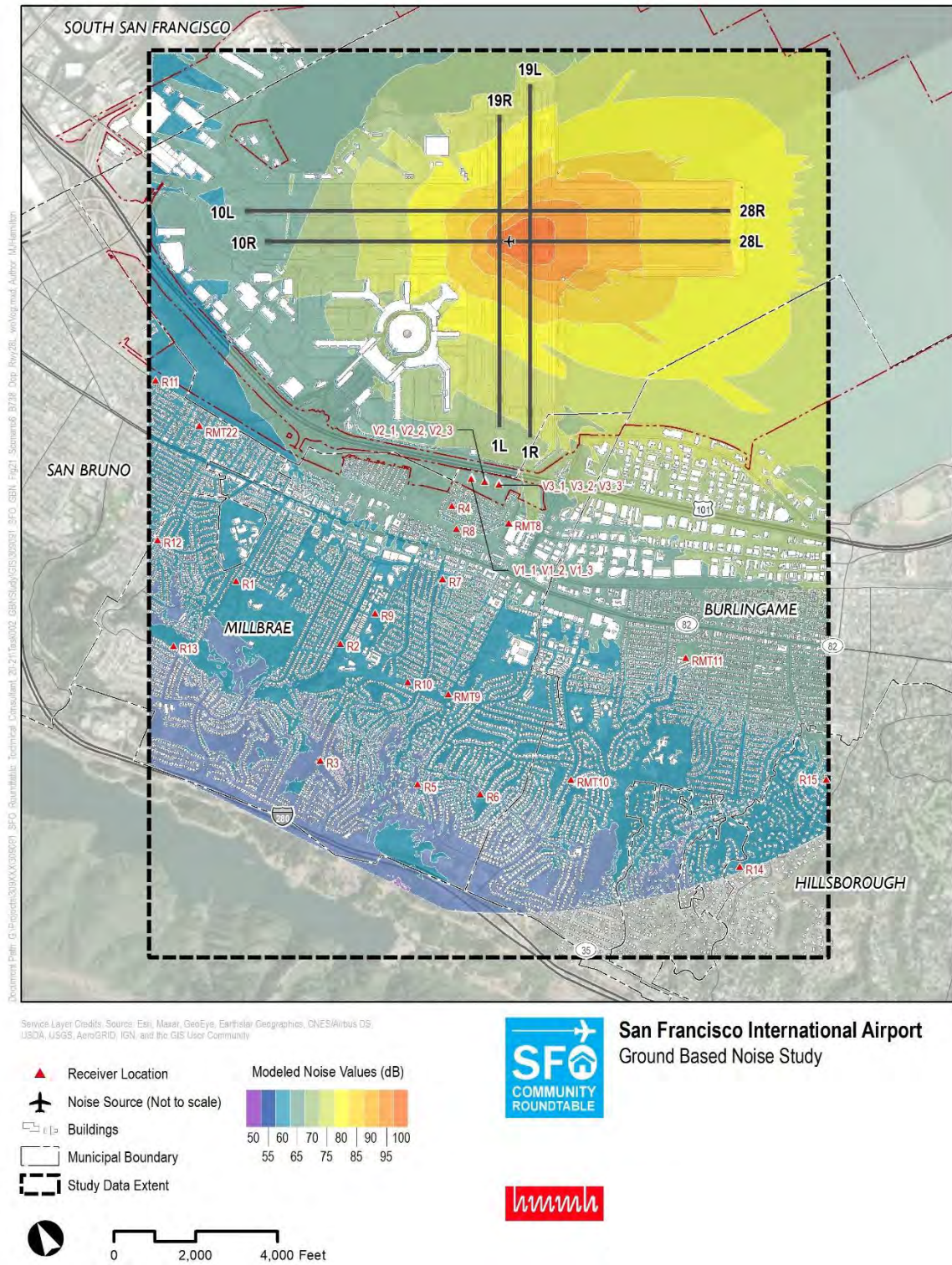
Figure 29: Scenario 6 – B77W Departing Runway 28L at Secondary Takeoff Point – Without Vegetation
