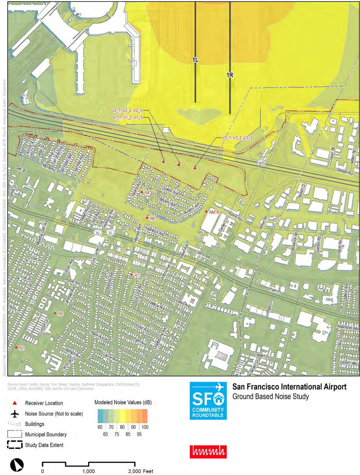
Figure H-13: Scenario 4 – B738 Departing Runway 1R at Secondary Takeoff Point – Without Vegetation
