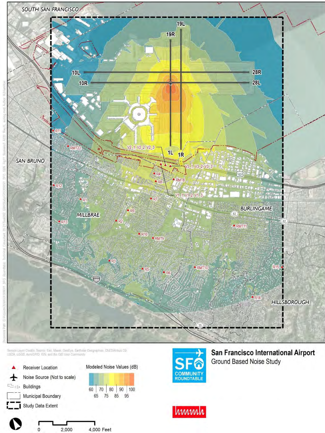
Figure 19: Scenario 3 – A320 Departing Runway 1L at Secondary Takeoff Point – Without Vegetation
