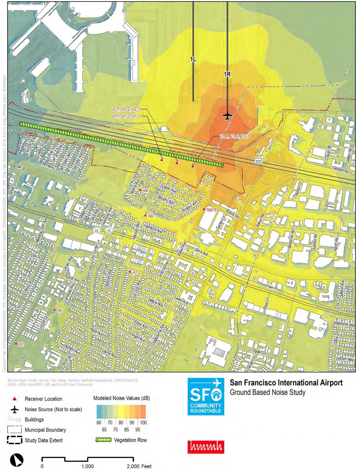
Figure H-6: Scenario 2 – B738 Departing Runway 1R at Start of Takeoff Roll – With Vegetation (50 Feet)
